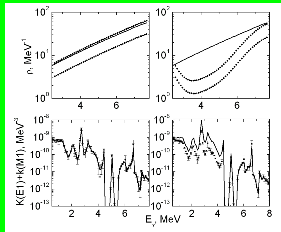
Fig. 7. Top row is fixed to the level density of ^{28}\text{Al} (points); lower – the best approximation of the radiative strength functions for fixed level density. Points with error bars – a standard presentation of radiation strength function, line - strength function in the equation (3).
