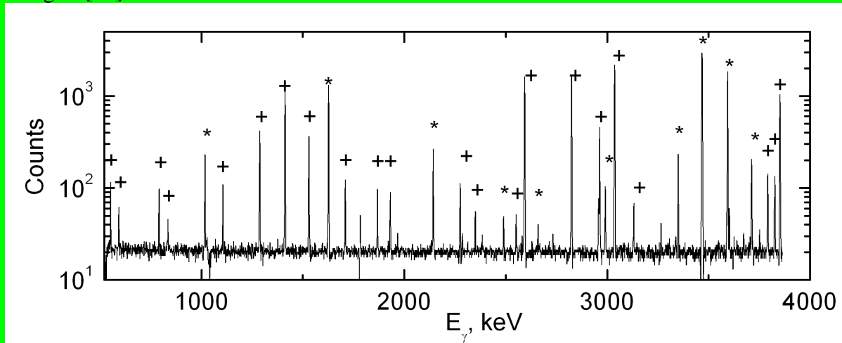
Fig. 2. Half the intensity distribution of two-step cascades on ground state. Crosses marked primary transition of ^{28}\text{Al} cascades, asterisks are secondary one's. Spectrum shifted up to 20 counts.
