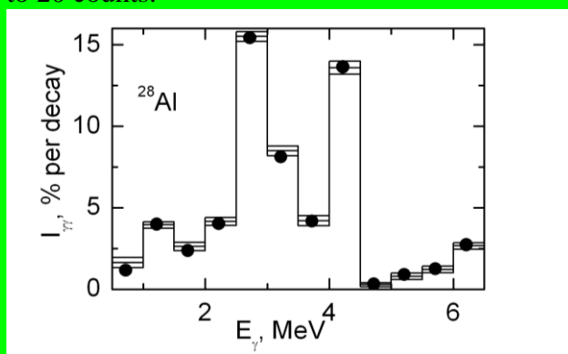
Fig. 3. Histogram - distribution of the intensity of the cascades to the 2 final level ^{28}\text{Al} in functions in their primary transition energy. Points are noted approximated value I_{\gamma\gamma} for one of the variants to define the random radiative strength and level density functions.
