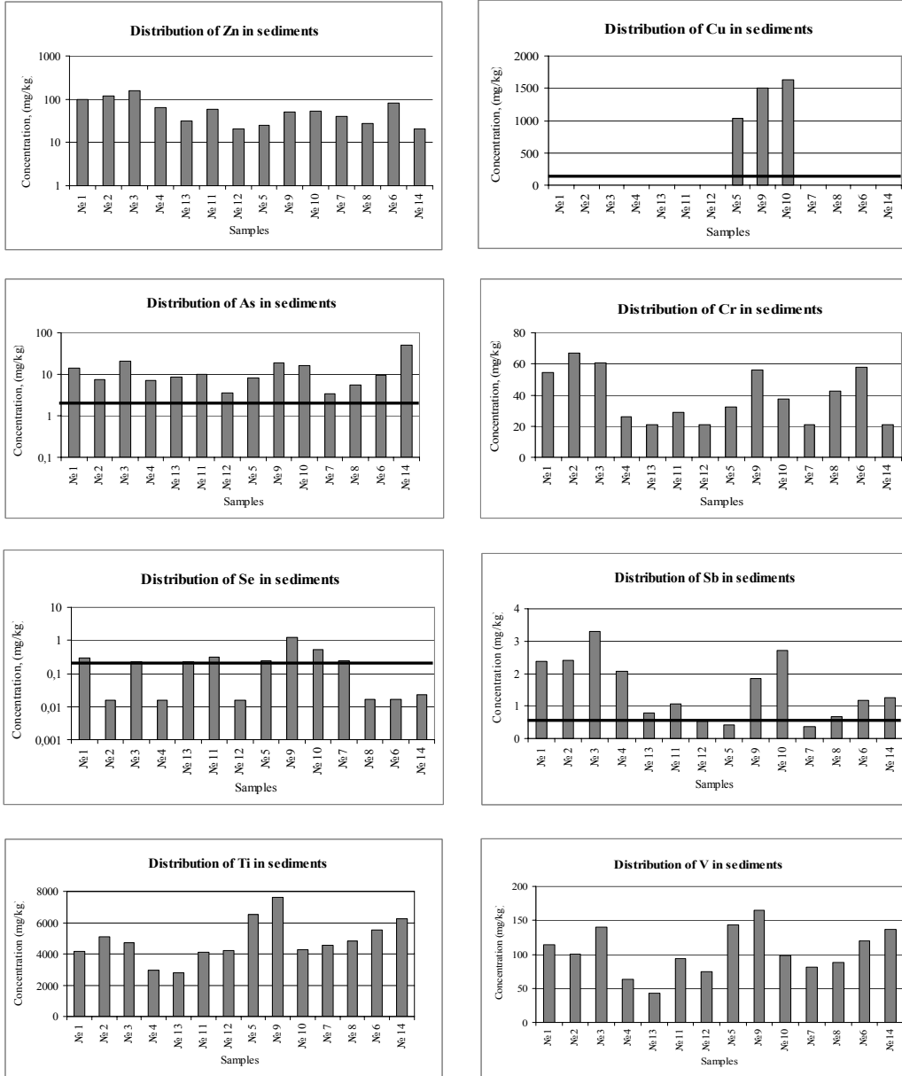
Fig. 2. Histogram of distribution for some micro elements in sediments
