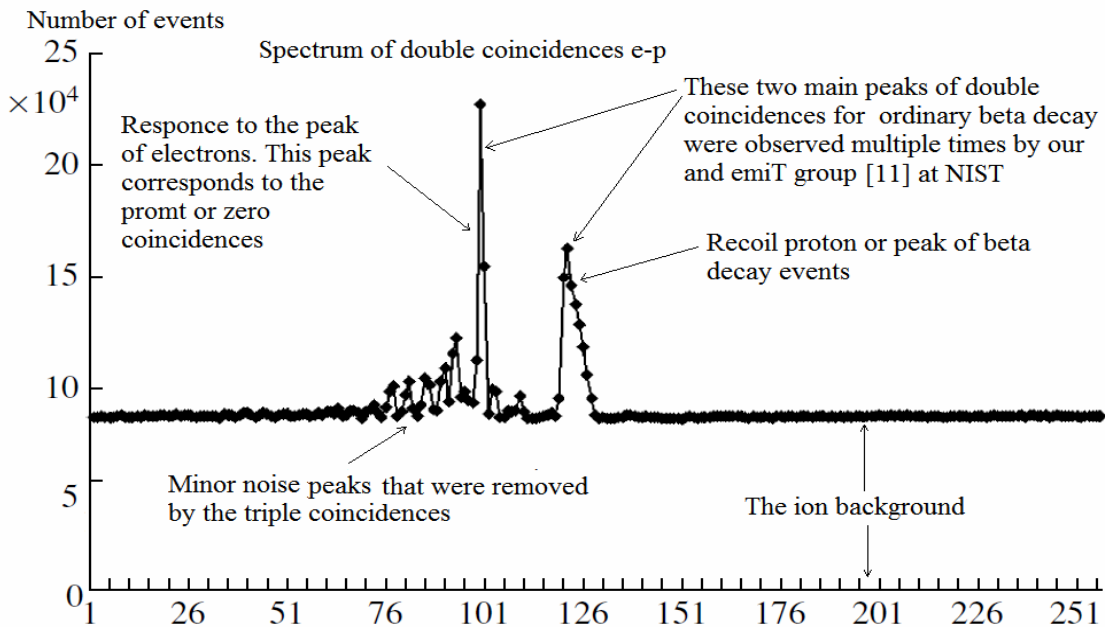
Fig. 1. Timing spectrum for e-p coincidences. Each channel corresponds to 25 ns. The peak at channel 99-100 corresponds to the prompt (or zero) coincidences. The coincidences between the decay electrons and delayed recoil protons (e-p coincidences) are contained in the large peak centered at channel 120.
