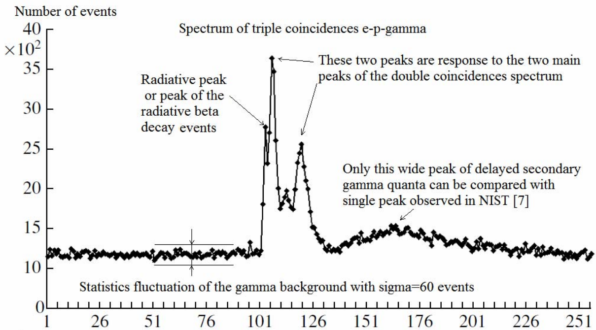
Fig. 5 Timing spectrum for triple e-p-g coincidences. Each channel corresponds to 25 ns. In this spectrum, three main peaks in channels 103, 106 and 120 can be distinguished. The leftmost peak in 103 channel among these three main peaks is connected with the peak of radiative decay events.
