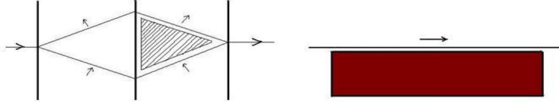
Figure 2: Left – scheme of the interferometric experiment to search for new spin-dependent forces, right – neutron spin rotation or beam deflection experiment.
