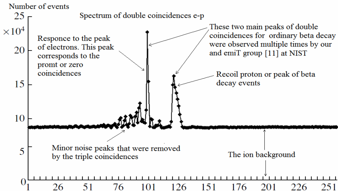
Fig. 1. Timing spectrum for e-p coincidences. Each channel corresponds to 25 ns. The peak at channel 99-100 corresponds to the prompt ( or zero ) coincidences. The coincidences between the decay electrons and delayed recoil protons (e-p coincidences) are contained in the large peak centered at channel 120.
