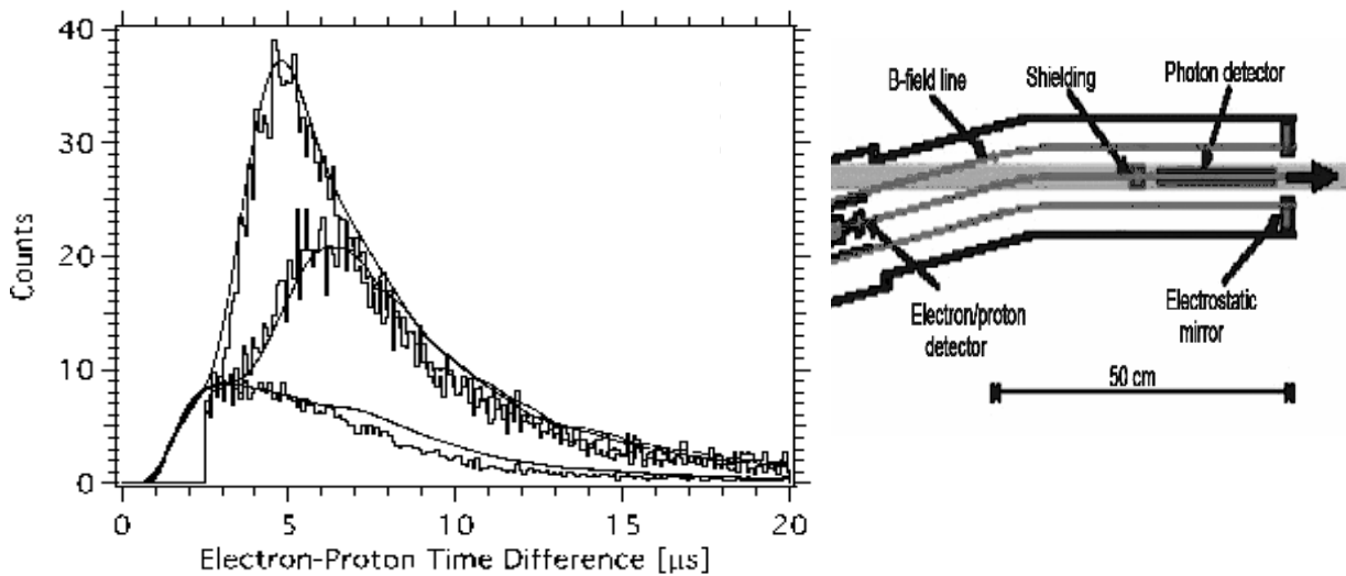
Fig. 3 Equipment diagram and the single peak of “electron-proton” coincidences, published in [13]. The location of the peak’s maximum and its significant width differ from our and the emiT results subsequently by one and two orders of magnitude. The location and the width of the peak also deviate by one and two orders of magnitude from the elementary estimates of delay times (see below).
