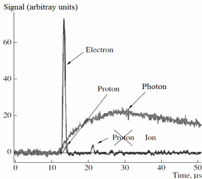
Fig. 4. The signal from the decay proton has to be delayed by less than one microsecond, which is why it is located at the base of the electron pulse ( see line number 2 ) and so cannot be registered by the combined electron-proton detector. The pulses that are delayed by longer than 1 microsecond are pulses not from decay protons, as it was indicated in ref. [7], but rather from ions, formed in the decay zone. The line number 1 shows the shape of pulses from the gamma detector
