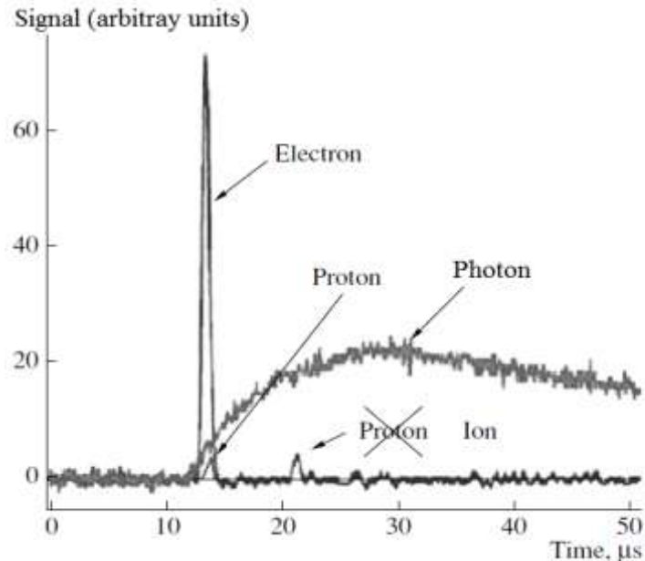
Fig.4. The signal from the decay proton has to be delayed by less than one microsecond, which is why it is located at the base of the electron pulse (see line number 2) and so cannot be registered by the combined electron-proton detector. The pulses that are delayed by longer than 1 microsecond are pulses not from decay protons, as it was indicated in ref. [7], but rather from ions, formed in the decay zone. The line number 1 shows the shape of pulses from the gamma detector.
