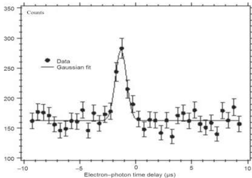
Fig.6. Only peak of “electron-photon” coincidences, shifted to the left of 0 – the time of beta-electron registration – by 1.25 microseconds, published in [7].
