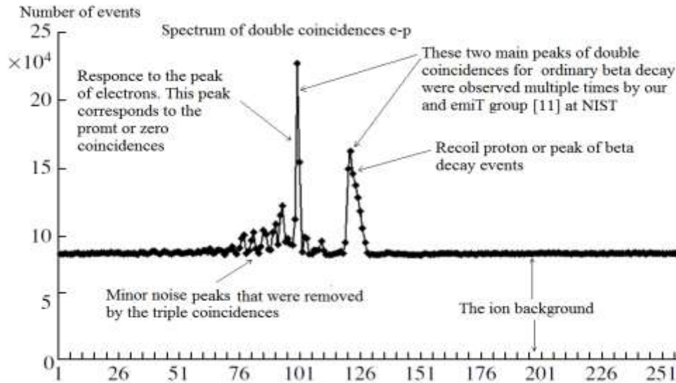
Fig.1. Timing spectrum for e-p coincidences. Each channel corresponds to 25 ns. The peak at channel 99-100 corresponds to the prompt (or zero) coincidences. The coincidences between the decay electrons and delayed recoil protons (e-p coincidences) are contained in the large peak centered at channel 120.
