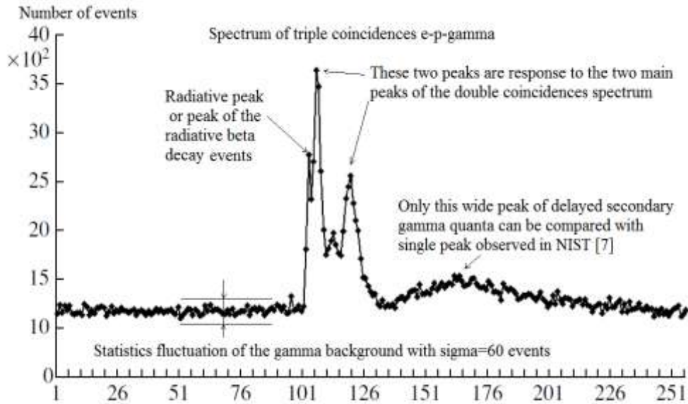
Fig.5. Timing spectrum for triple e-p-g coincidences. Each channel corresponds to 25 ns. In this spectrum, three main peaks in channels 103, 106 and 120 can be distinguished. The leftmost peak in 103 channel among these three main peaks is connected with the peak of radiative decay events.
