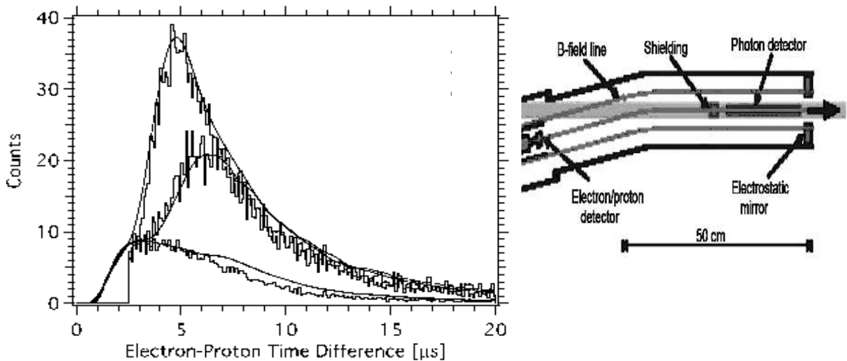
Fig.3. Equipment diagram and the single peak of “electron-proton” coincidences, published in [13]. The lower curve corresponds to 0 volts, the middle curve corresponds to 300 volts and the highest curve corresponds to 500 volts in an electrostatic mirror.
