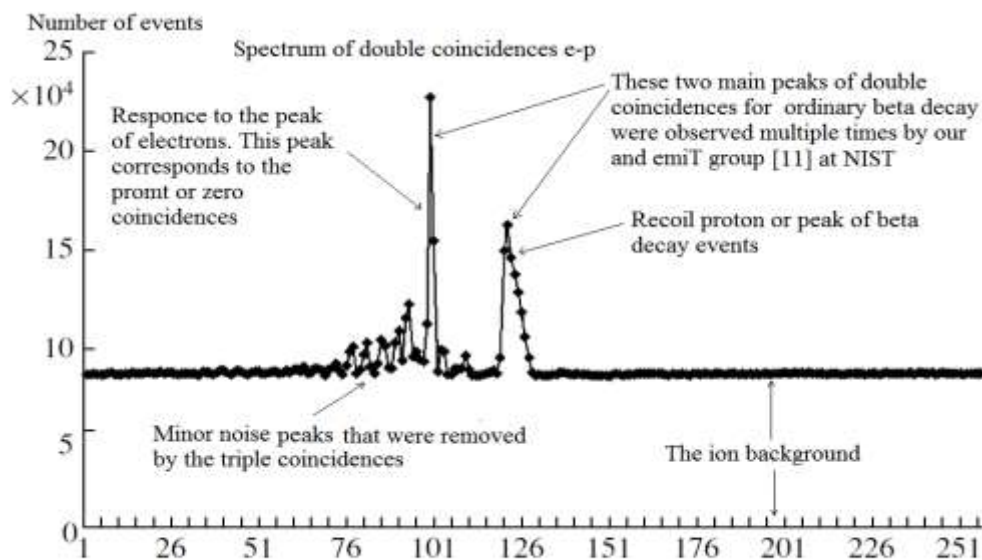
Fig.2. Timing spectrum for e-p coincidences. Each channel corresponds to 25 ns. The peak at channel 99-100 corresponds to the prompt (or zero) coincidences. The coincidences between the decay electrons and delayed recoil protons (e-p coincidences) are contained in the large peak centered at channel 120.
