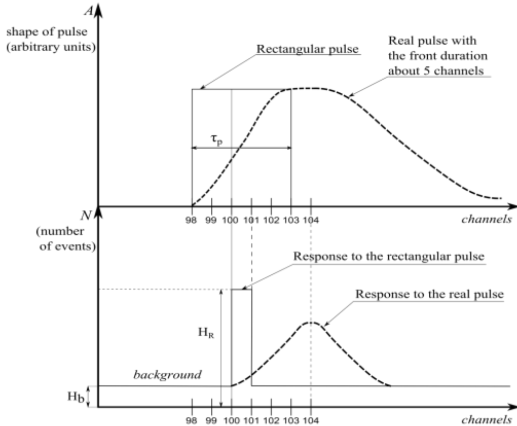
Fig.1. The top graph presents the shape of the impulses. The flat line shows the rectangular impulse with a zero front duration, while the dotted line represents the real front duration. The lower graph presents the form of the response peaks in time spectrum: the flat line shows the ideal case of rectangular impulses and the dotted line shows the real impulses.
