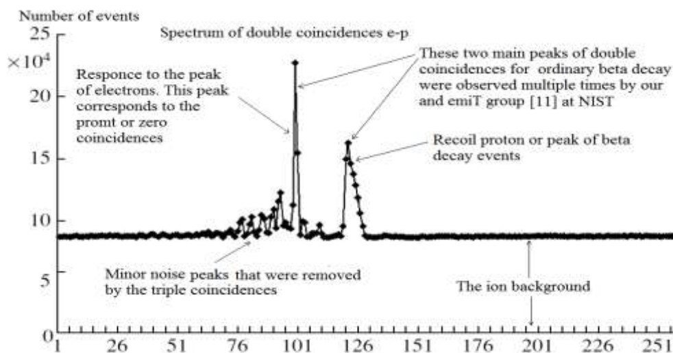
Fig. 2. Timing spectrum for e-p coincidences. Each channel corresponds to 25 ns. The peak at channel 99–100 corresponds to the prompt (or zero) coincidences. The coincidences between the decay electrons and delayed recoil protons (e-p coincidences) are contained in the large peak centered at channel 120.
