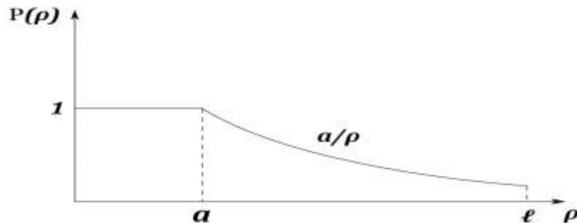
Fig. 1. The dependence of the ionization probability on \rho . For the usual model: P(\rho)=1 for \rho < a and P(\rho)=0 for a < \rho < \ell ; for Coulomb interaction model P(\rho) = 1 and P(\rho) = a/\rho for a < \rho < \ell .
