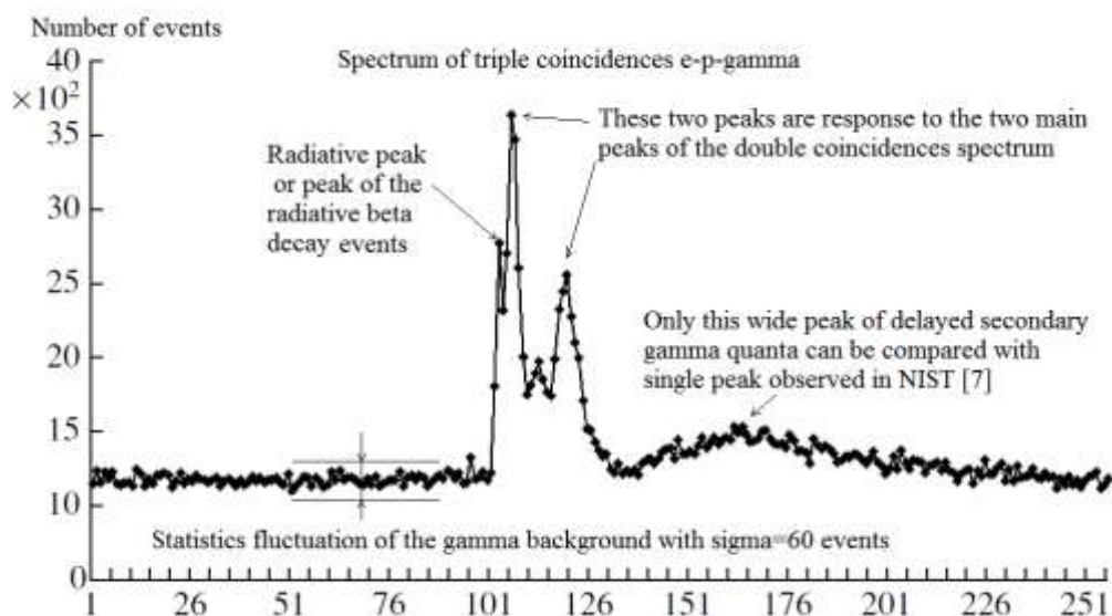
Fig. 6. Timing spectrum for triple e-p-g coincidences. Each channel corresponds to 25 ns. In this spectrum, three main peaks in channels 103, 106 and 120 can be distinguished. The left most peak in 103 channel among these three main peaks is connected with the peak of radiative decay events.
