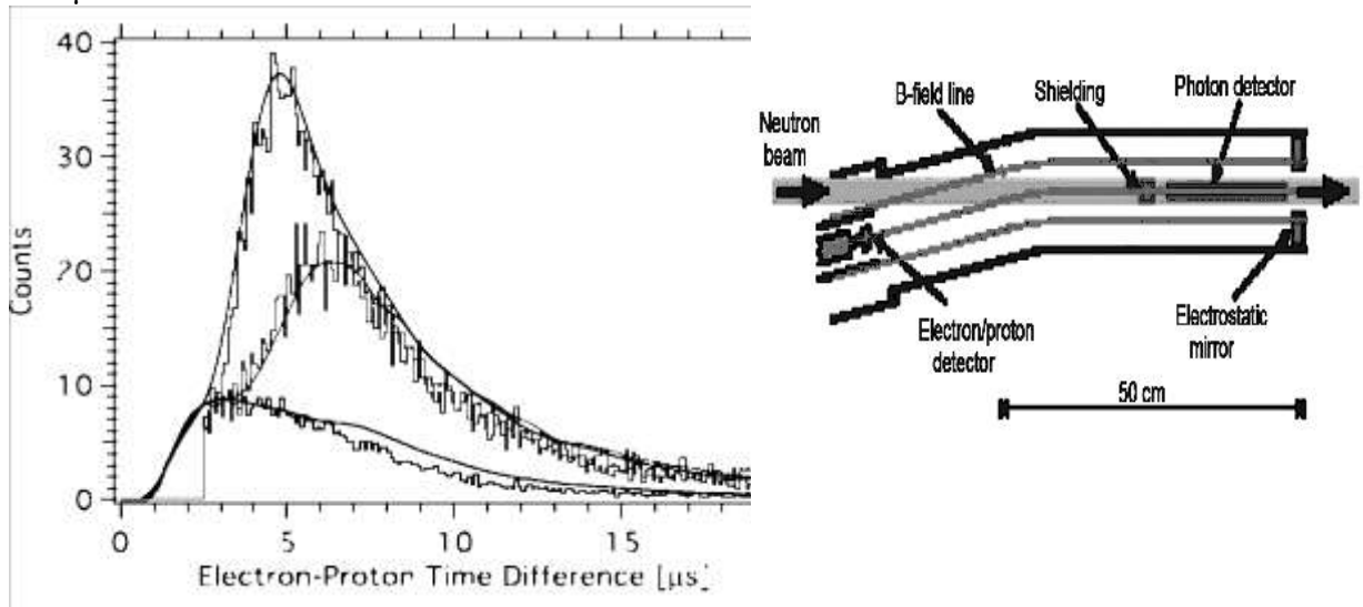
Fig. 4. Equipment diagram and the single peak of "electron-proton" coincidences, published in [13]. The lower curve corresponds to 0 volts, the middle curve corresponds to 300 volts and the highest curve corresponds to 500 volts in an electrostatic mirror. The location of the peak's maximum and its significant width differ from our and the emiT results subsequently by one and two orders of magnitude. The location and the width of the peak also deviate by one and two orders of magnitude from the elementary estimates of delay times (see below).
