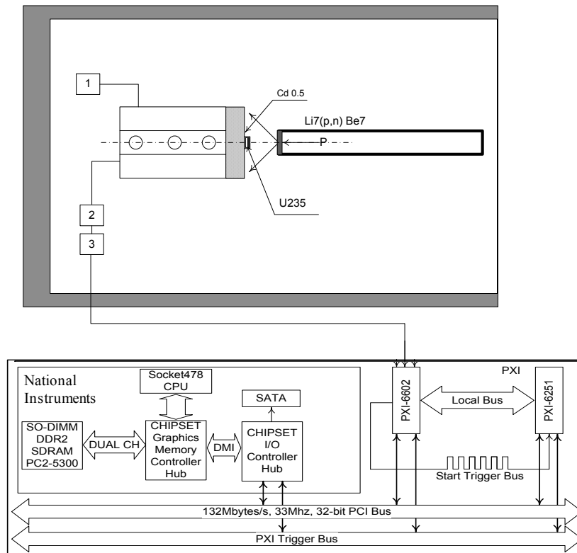
1 – high voltage source; 2 – preamplifiers of signals from the counters SNM-18; 3 – summator of signals from the preamplifier of detector counters.
