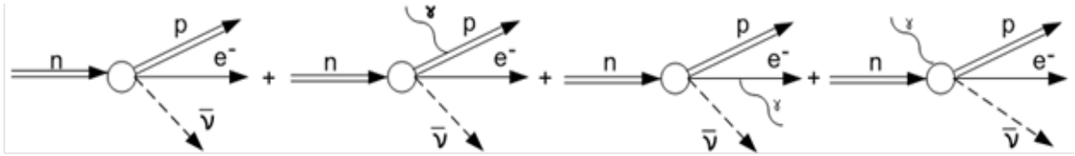
Fig.1. The Feynman diagrams describing neutron decay. Last one describes the emission of structure gammas.
